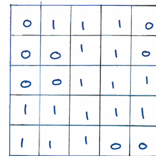
The induced matrix f_0
