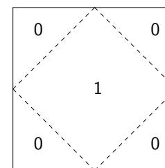
Figure: An approximate shape of the matrix for a cycle with maximal entropy.
