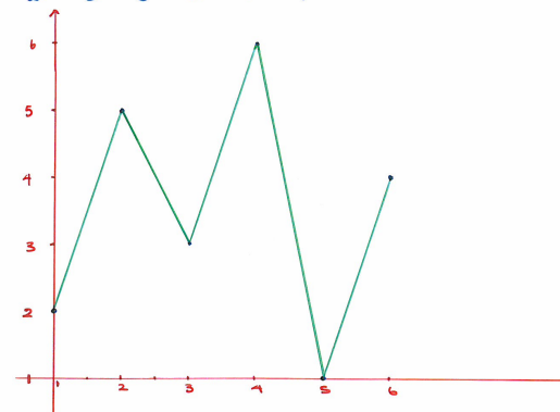
The graph of f_\theta .
