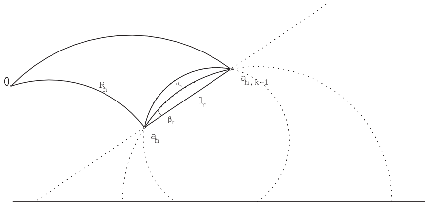
Figure 3. A triangle forming the \lambda -polygon K_n .
