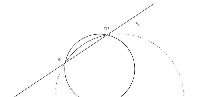
Figure 2. \lambda -geodesic segments with end points A and B' .
