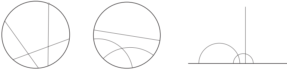
Figure 1. Hyperbolic plane models: projective, disk and half-plane.
