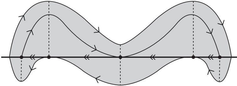
FIGURE 10. Non-trivial minimal set presenting non-empty interior.
