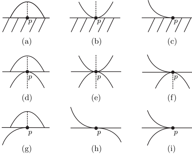
FIGURE 2. Cases where occur regular tangential singularities. The dashed lines represent the curves where X.f(p) = 0 or Y.f(p) = 0 .
