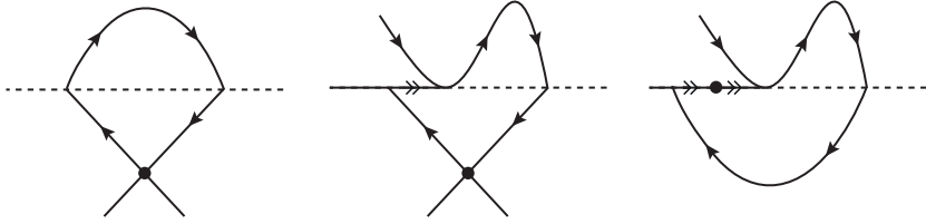
FIGURE 6. Examples of pseudo-graphs.
