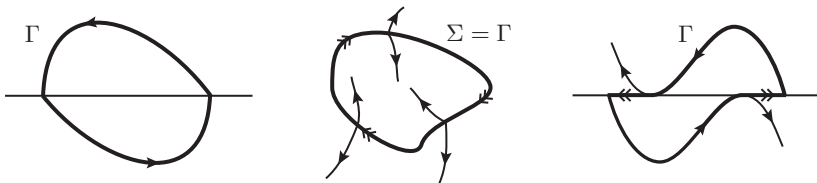
FIGURE 5. Possible kinds of pseudo-cycles.
