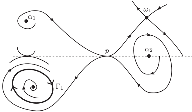
FIGURE 8. Both the \alpha -limit set \{\alpha_1, \alpha_2\} and the \omega -limit set \{\omega_1, \Gamma_1\} of the point p are disconnected. Sliding motion on \Sigma is not allowed.
