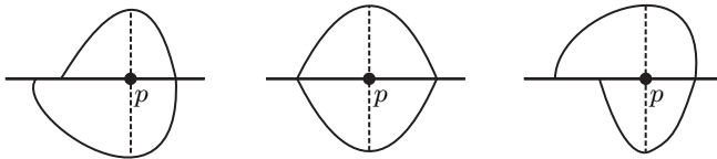
FIGURE 3. The particular cases where occur singular tangential singularities.
