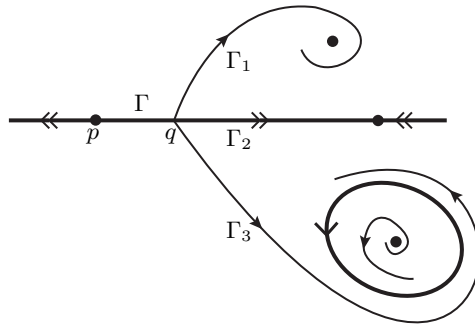
FIGURE 4. An orbit by a point is not necessarily unique.
