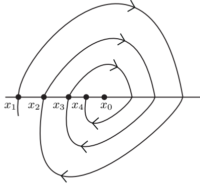
FIGURE 7. Case where there exists a singular tangency in \omega(\Gamma_Z(t, p)) \cap \Sigma .
