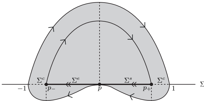
FIGURE 9. Special integral curves and tangency points.
