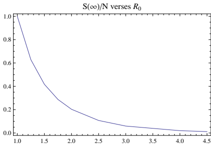
Figure 4: Plot of S(\infty)/N versus R_0 .
