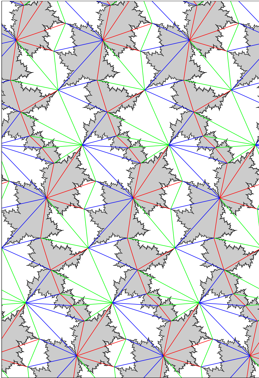
FIGURE 1. Projected-horosphere triangulation \Delta(\varphi) and fractal tessellation CW(\varphi) , for \varphi = RLLRRRLLLL . The straight line segments etch \Delta(\varphi) while the fractal lines etch CW(\varphi) .
